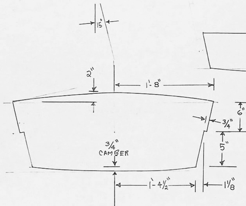
TRANSOM SCALE 1 1/2"=1'
