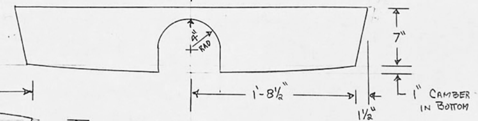
MIDSHIPS FRAME SCALE 1 1/2"=1'
